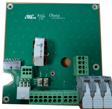
PCBa OFP PSU CONNECTOR (48Vdc)
