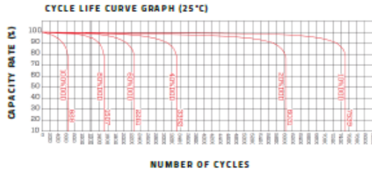
CYCLE LIFE CURVE GRAPH
