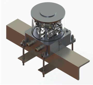
OFC bracket for horizontal bracket
